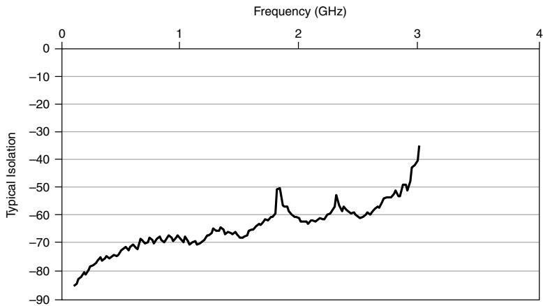
Figure 3. Typical Isolation
